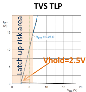
5V TVS with V_{hold} = 2.5V
